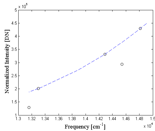
Figure 21. Plot of the normalized intensities measuring the sun through each filter with the baseline fit to the three out-of-band filters used. The two points below the curve are the normalized intensities for the in-band filters. The one on the far left is the NIR band and the one on the right is the visible band.
